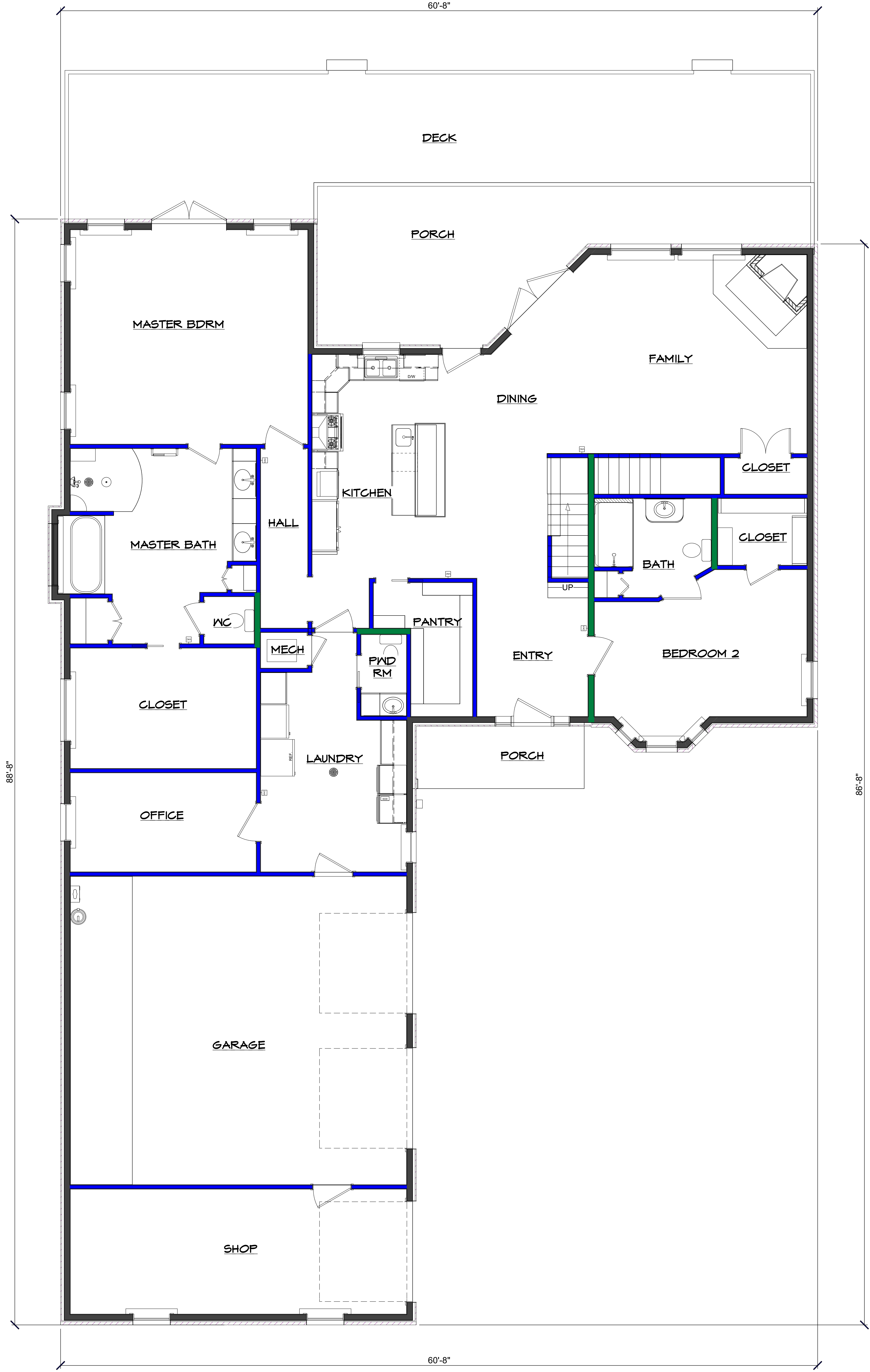
First Floor Plan
