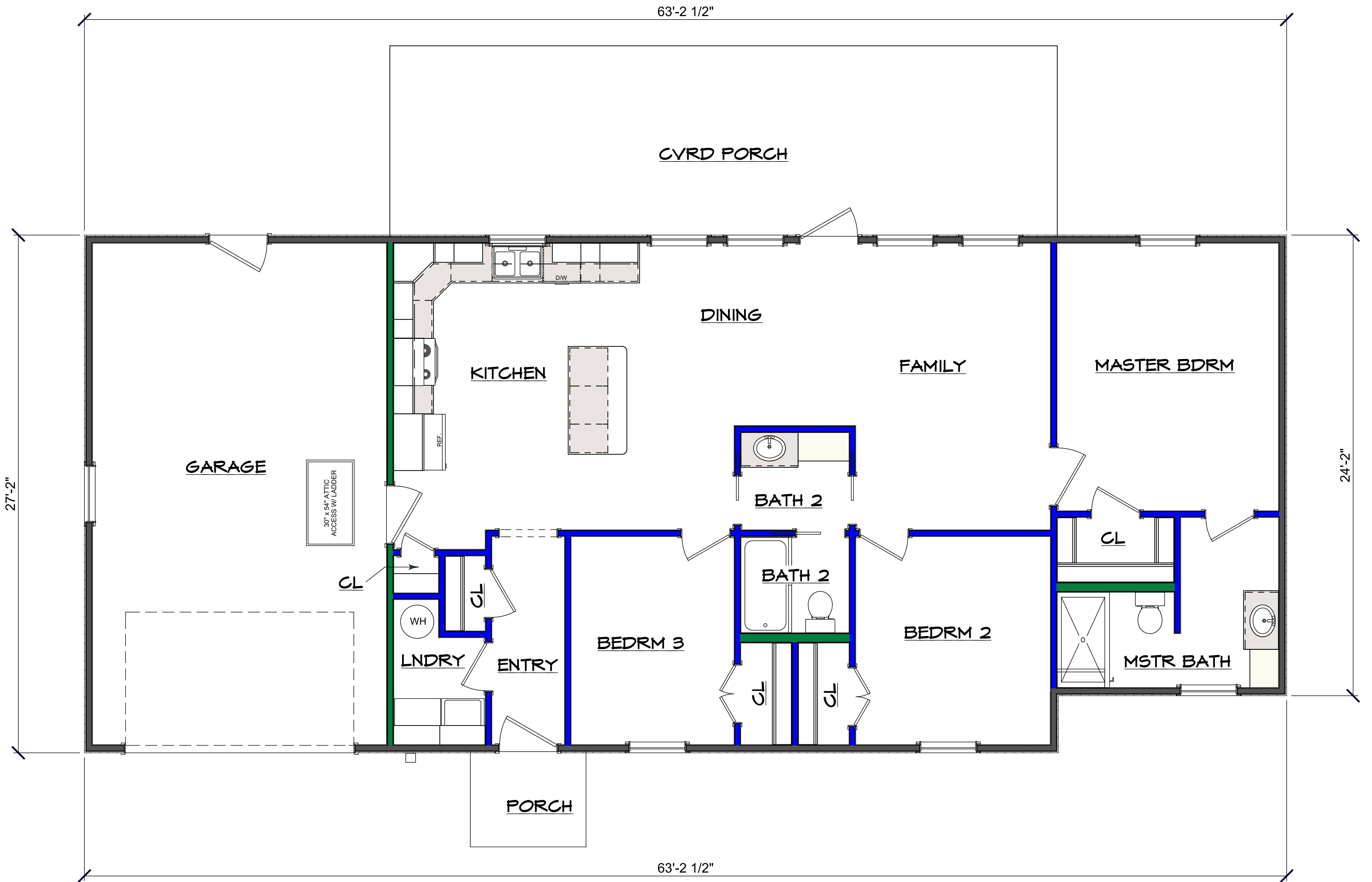
First Floor
